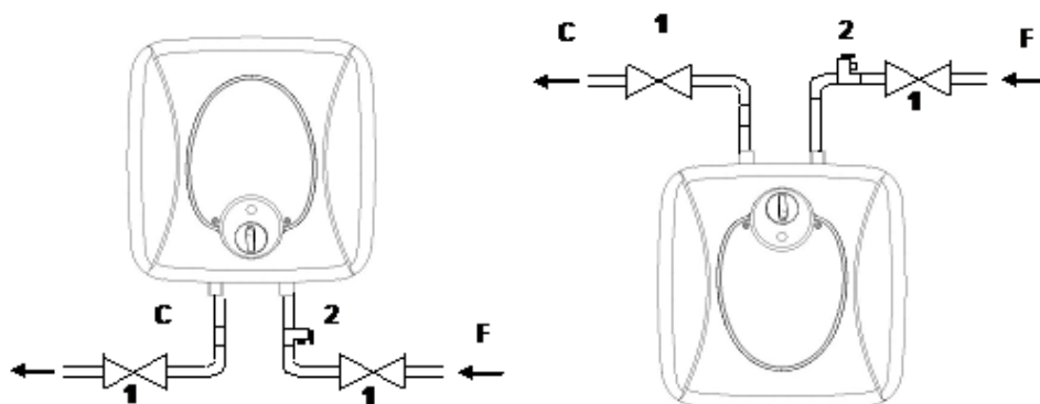
Fig-3 Installation hydraulique
