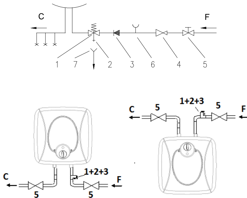
Fig-2 Hydraulic installation
