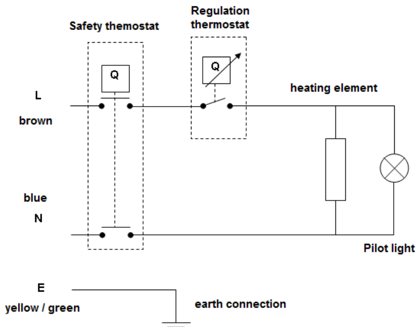
Fig. – 4 APARICI – SB15 electrical diagram.
